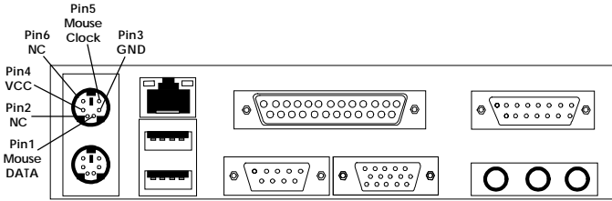
PS/2 Mouse (6-pin Female)
