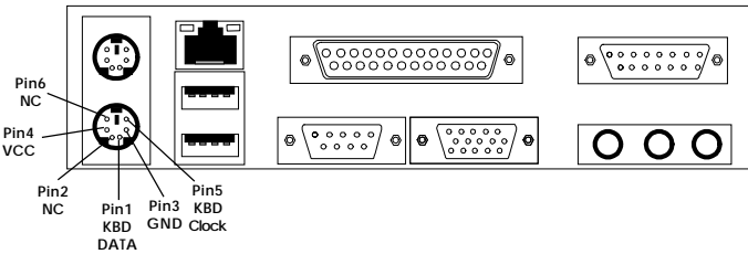
PS/2 Keyboard (6-pin Female)
