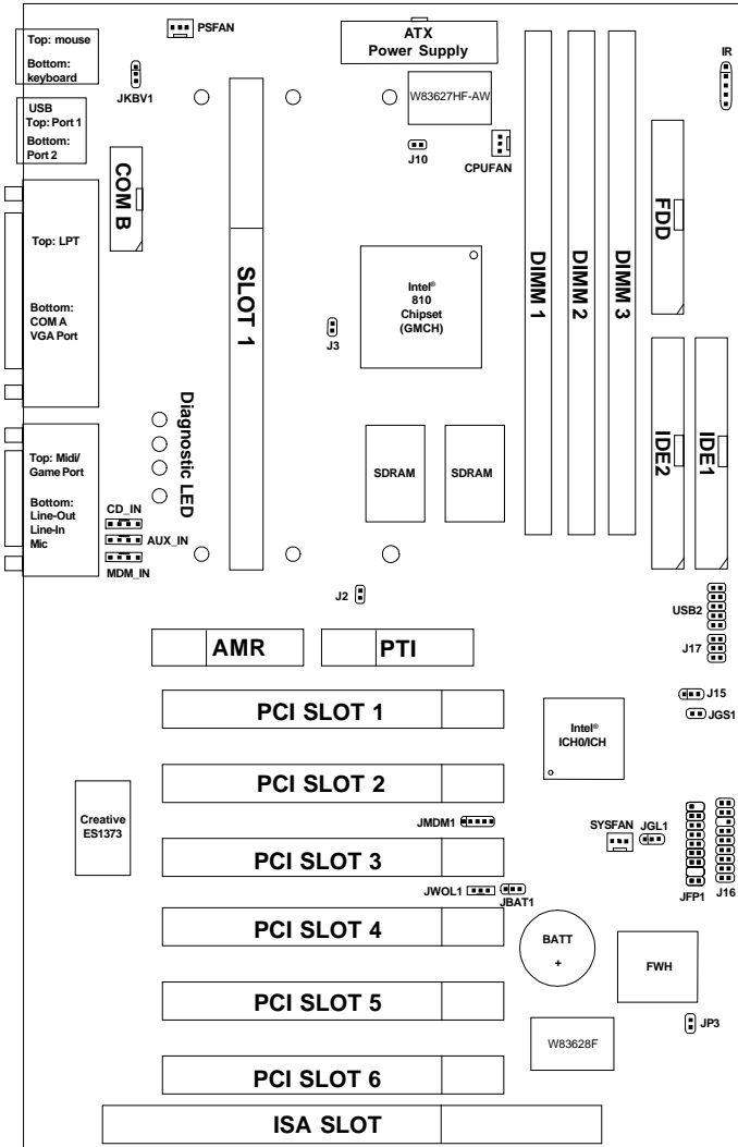
MS-6182 ATX WH8 Mainboard
