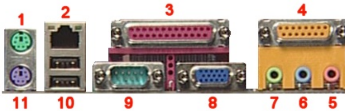
Figure 2: Backplate
