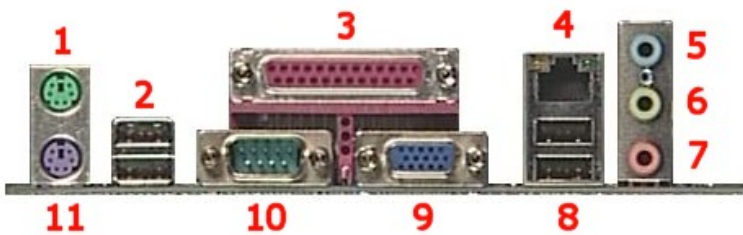
Figure 3: Backplate
