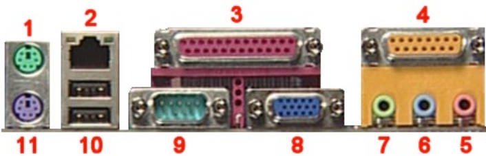
Figure 2: Backplate
