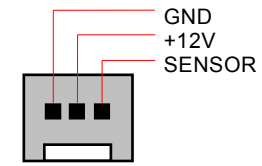
SYSFAN2 Connector
