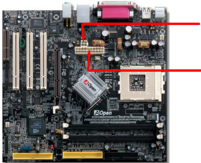
4-pin 12V. ATX Power
