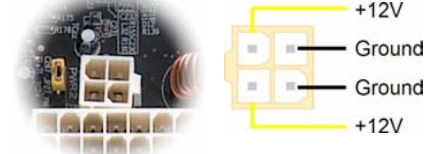
4-pin 12V. ATX Power
