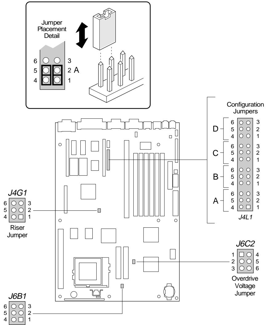
Figure 6. Jumper Locations
