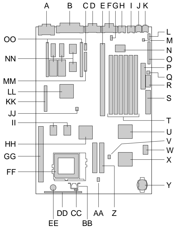
Figure 1. Motherboard Components
