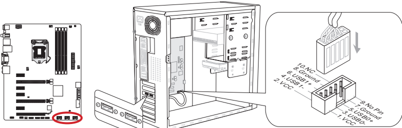
USB 2.0 Slotblech (optional)
