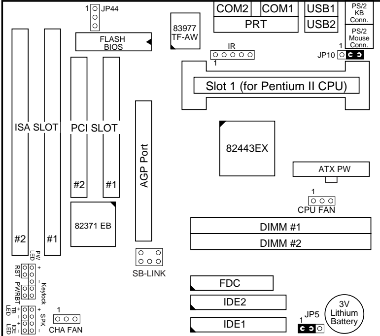
Figure 1–2. Mainboard Default Setting
