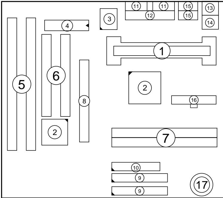
Figure 1-1. Mainboard Layout
