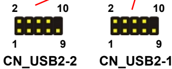
CN_USB 2-1/2-2: USB2.0 10-pin header
