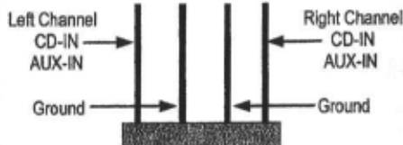
Front View of a CD/AUX-IN Connector
