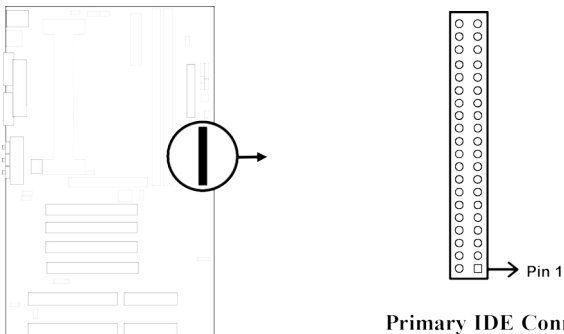
Primary IDE Connector
