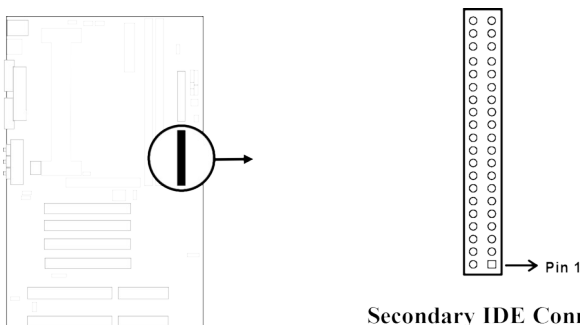
Secondary IDE Connector
