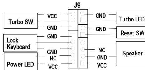
System Case Connections
