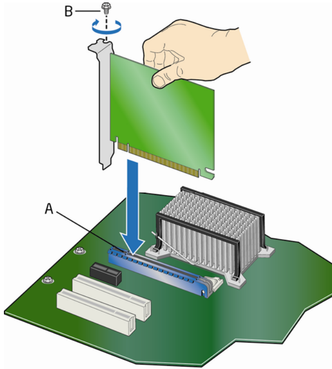
Figure 17. Installing a PCI Express x16 Card
