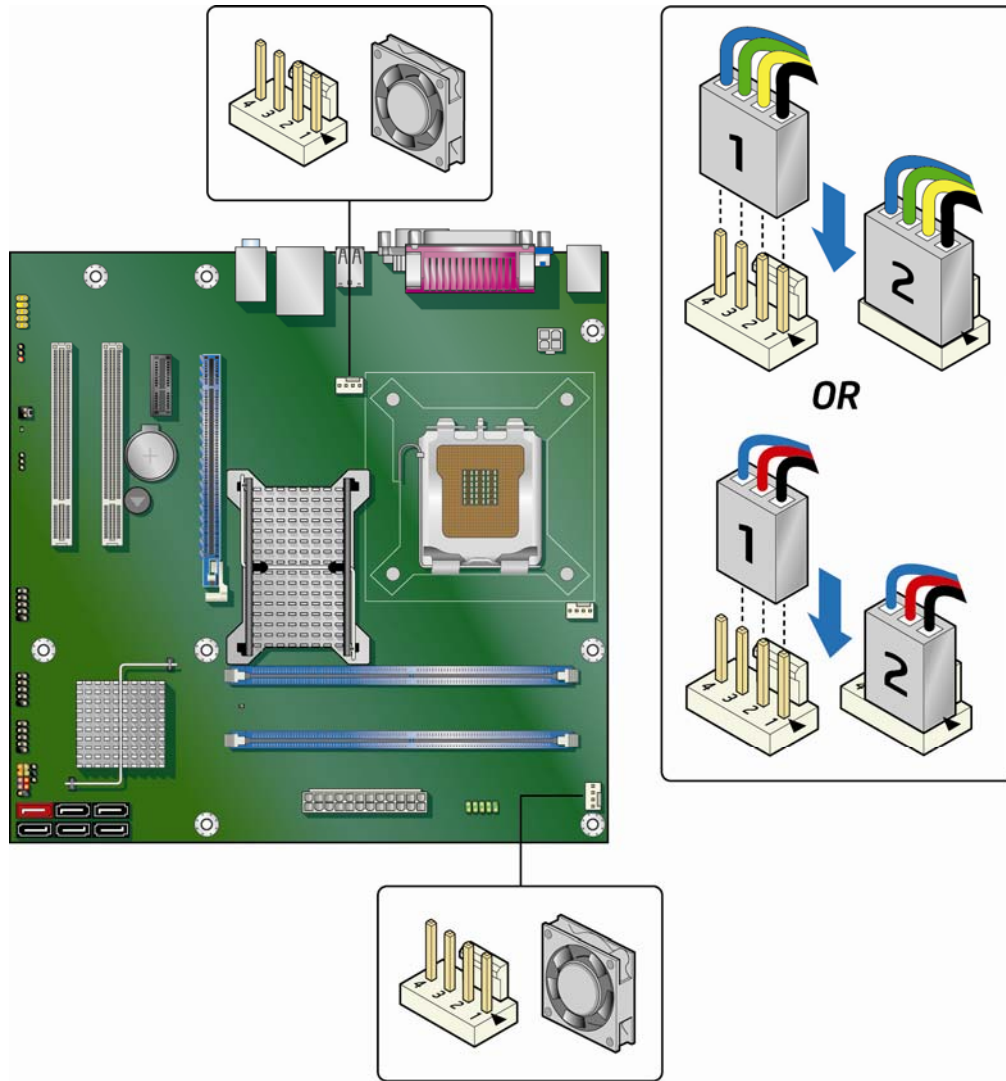
Figure 22. Location of the Chassis Fan Headers
