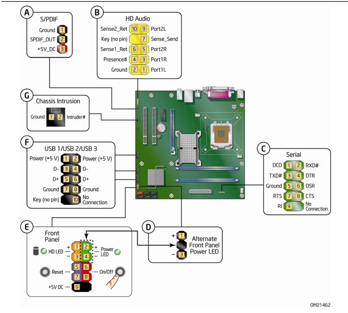
Figure 20. Internal Headers
