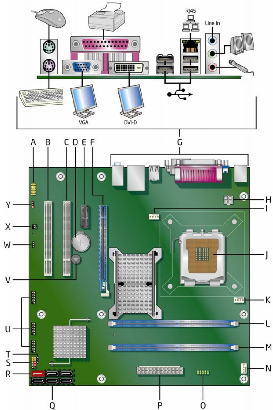
Figure 1. Intel Desktop Board DB43LD Components
