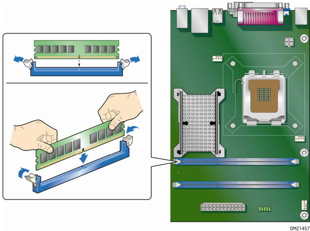
Figure 16. Installing a DIMM
