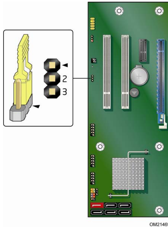
Figure 24. Location of the BIOS Configuration Jumper Block
