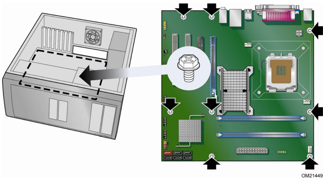
Figure 6. Intel Desktop Board DB43LD Mounting Screw Hole Locations
