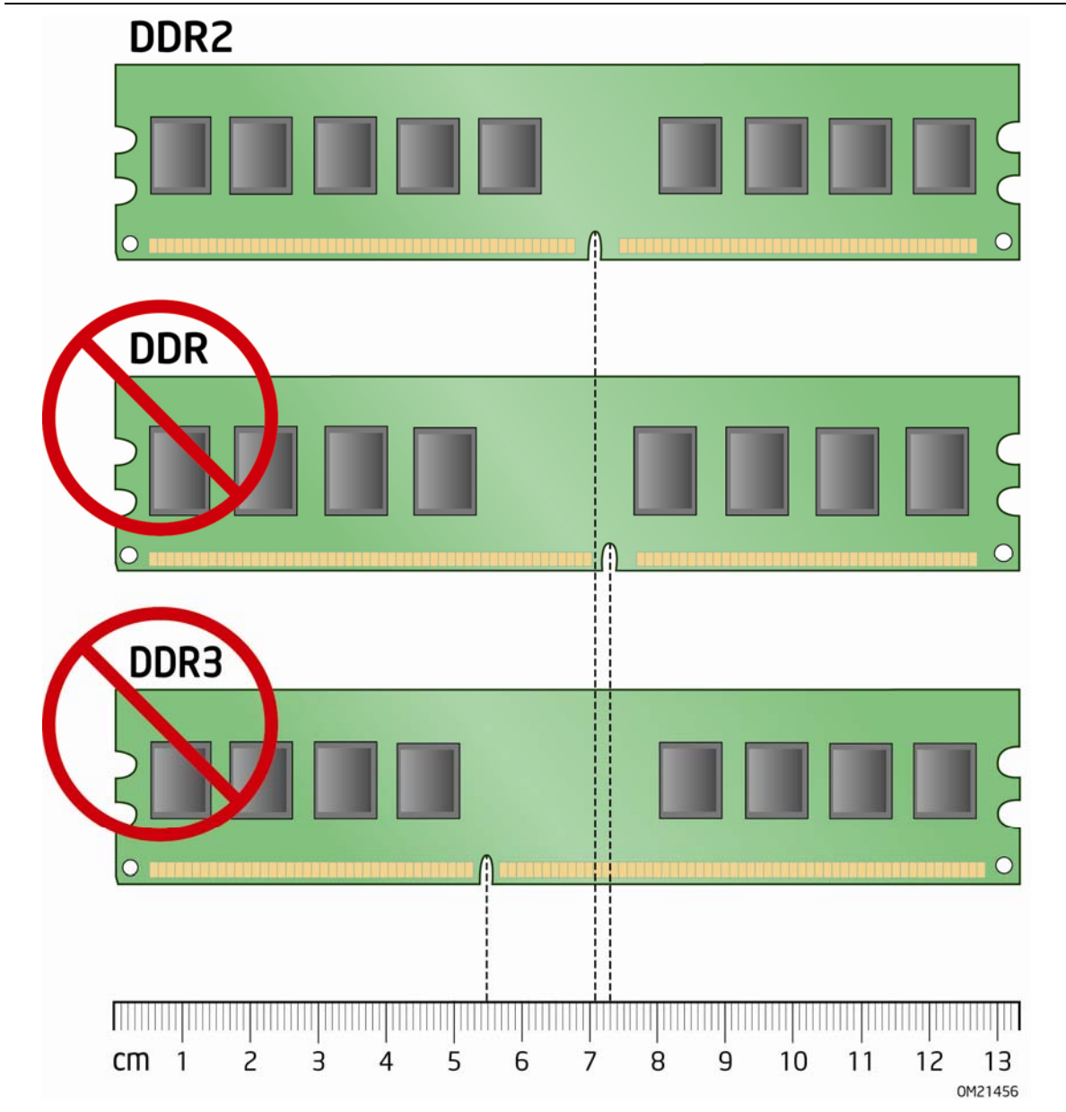
Figure 15. Use DDR2 DIMMs
