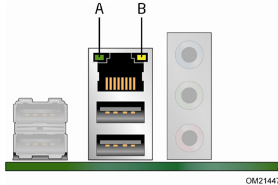
Figure 2. LAN Status LEDs
