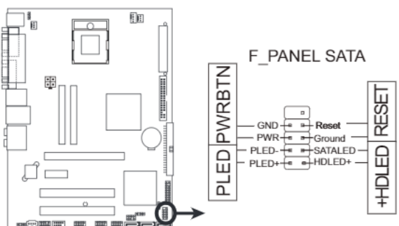
IMISR-VM FRONT PANEL CONNECTOR
