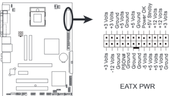
IMISR-VM EXTENDED ATX POWER CONNECTOR
