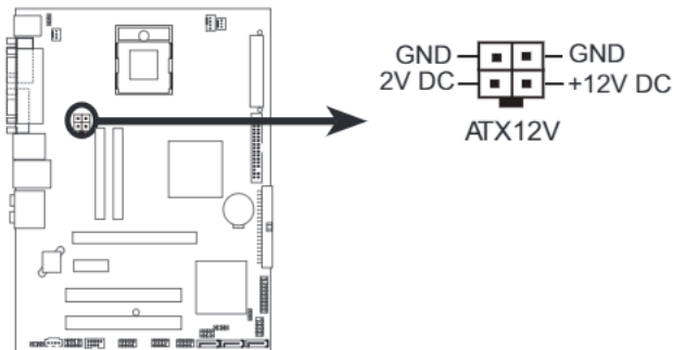
IMISR-VM ATX 12V POWER CONNECTOR
