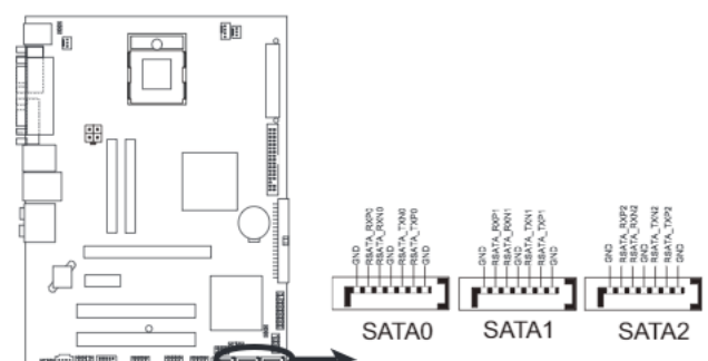
IMISR-VM SATA CONNECTORS
