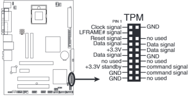
IMISR-VM INTERNAL TPM CONNECTOR
