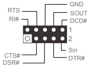
COM1 Connector (i945Ga-PHS Only)
