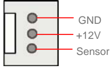
SYSFAN2 Connector
