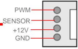
CPUFAN Connector
