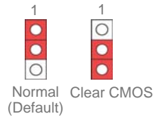
JP14 Clear CMOS Jumper
