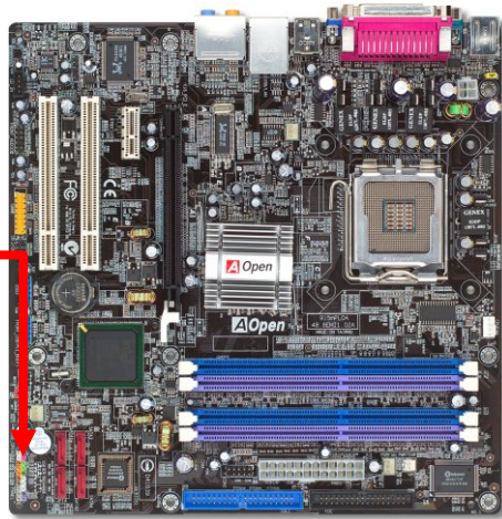
Front Panel Connector
