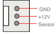
SYSFAN1 Connector
