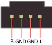
CD-IN Connector
