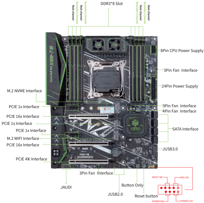
1-1 X99-T8 Gmotherboard Illustration
