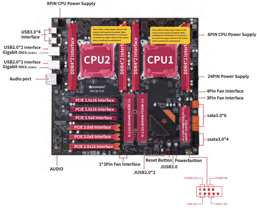
1-1 X99-F8D PLUS motherboard illustration
