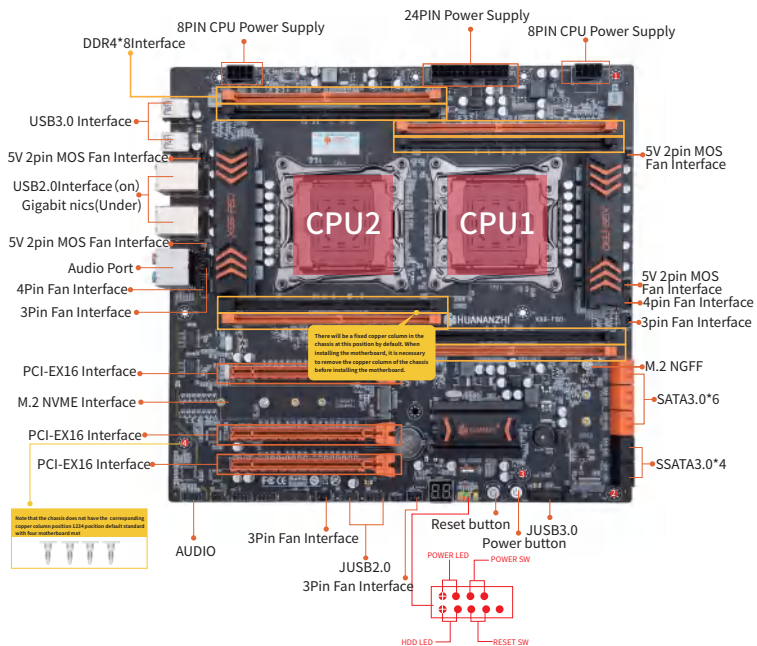
1-1 X99-F8D motherboard illustration
