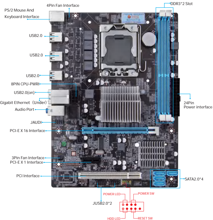
1-1 X58 2.0 motherboard illustration
