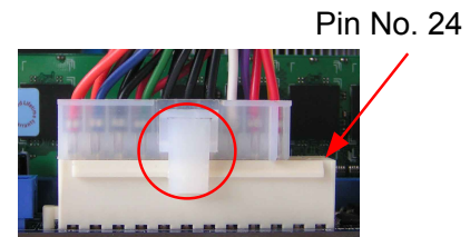
20-Pin Power
