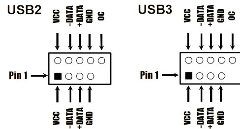
USB Port Headers
