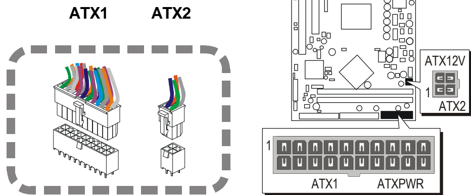
P4 ATX Power supply headers
