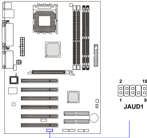
Pin Definition
