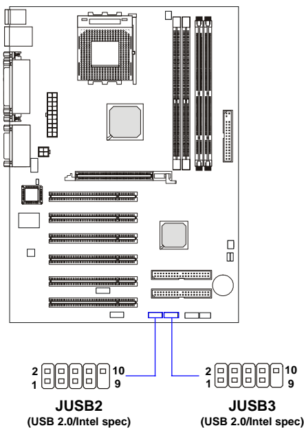
JUSB2/3 Pin Definition
