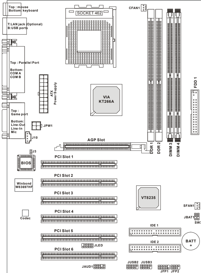
KT2 Combo (MS-6764 v1.X) ATX Mainboard
