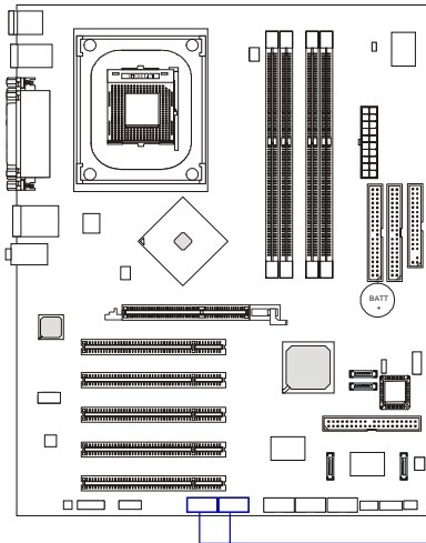
JUSB1 & JUSB2 Pin Definition
