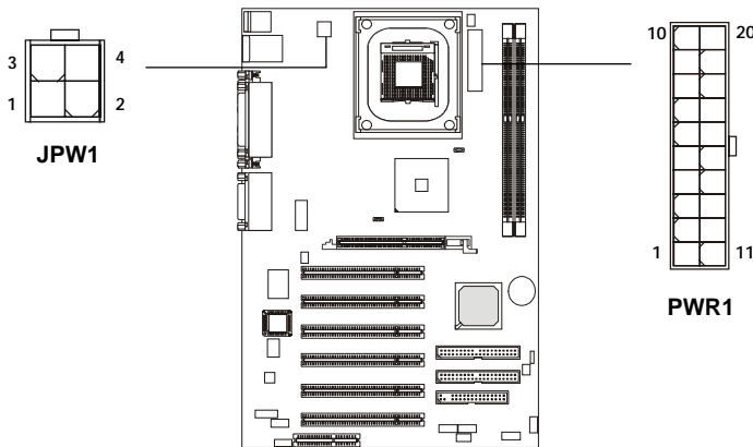
PWR1 Pin Definition
