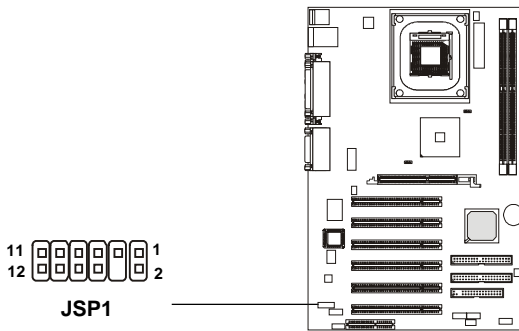
JSP1 Pin Definition
