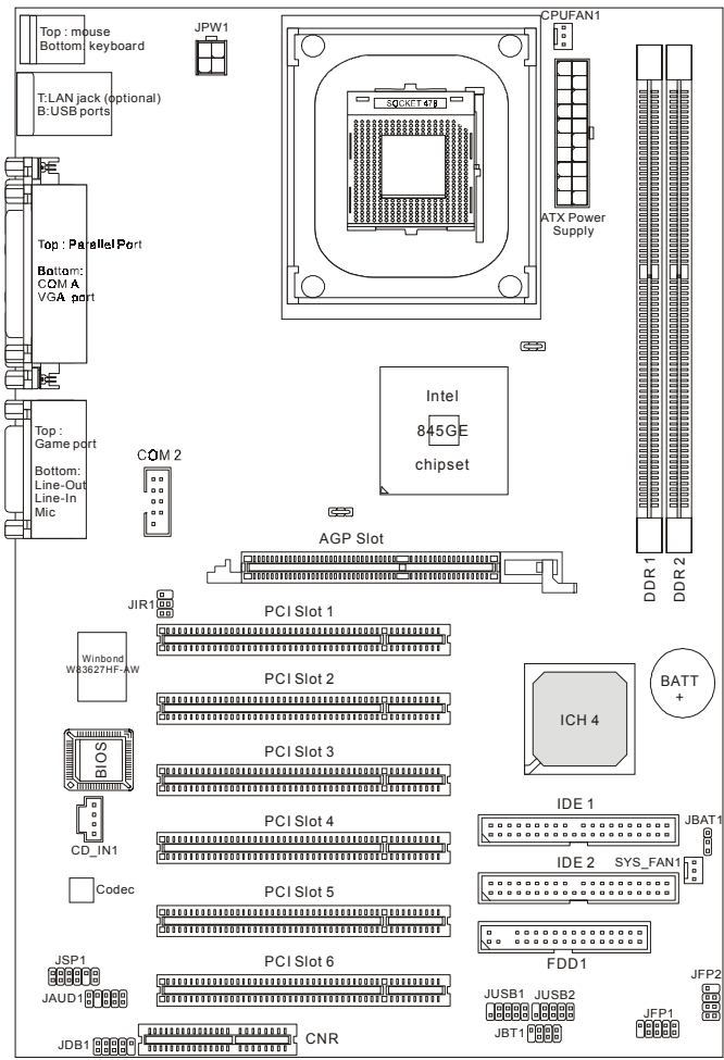
MS-6580 v2.X ATX Mainboard
