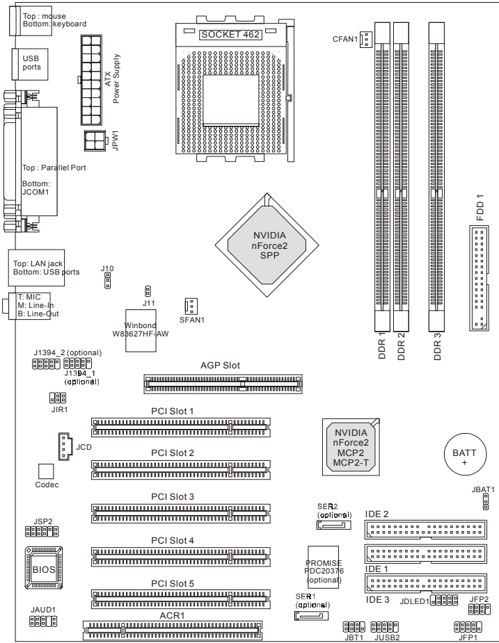
K7N2 Delta-L/LS/ILSR (MS-6570 v1.X) ATX Mainboard
