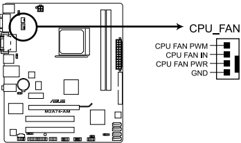
M2A74-AM CPU fan connector
