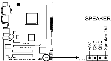
M2A74-AM Speaker Out Connector
