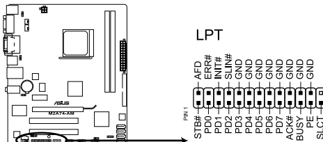
M2A74-AM Parallel Port Connector
