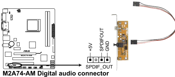
M2A74-AM Digital audio connector
