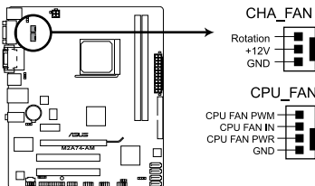
M2A74-AM fan connectors
