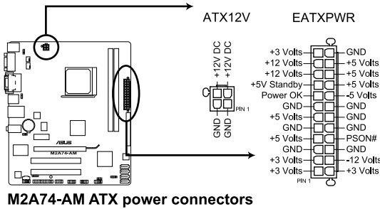
M2A74-AM ATX power connectors
