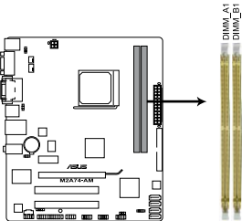
M2A74-AM 240-pin DDR2 DIMM sockets
