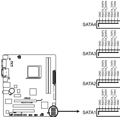
M2A74-AM SATA connectors
