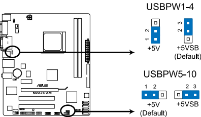
M2A74-AM USB Device Wake Up
