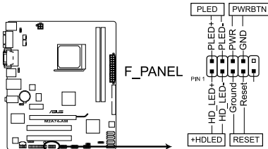
M2A74-AM System panel connector
