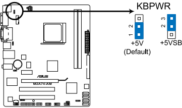
M2A74-AM Keyboard Power Setting
