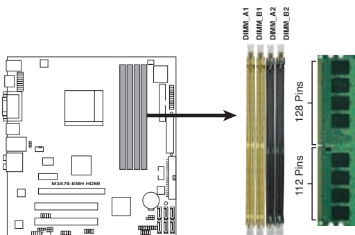
M3A78-EMH HDMI 240-pin DDR2 DIMM Sockets
