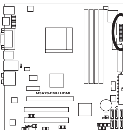
M3A78-EMH HDMI Parallel Port Connector
