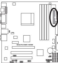
M3A78-EMH HDMI Floppy Disk Drive Connector
