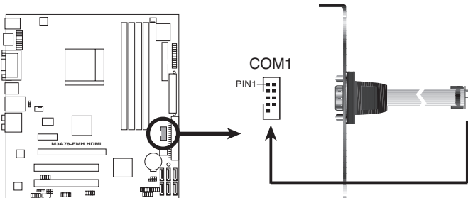
M3A78-EMH HDMI COM Port Connector
