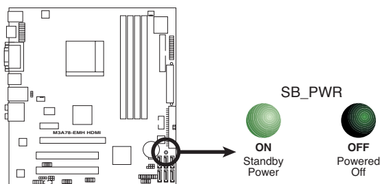
M3A78-EMH HDMI Onboard LED
