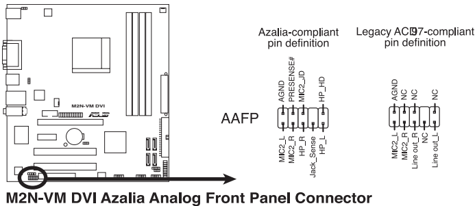
M2N-VM DVI Azalia Analog Front Panel Connector
