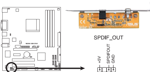
M2N-VM DVI Digital Audio Connector
