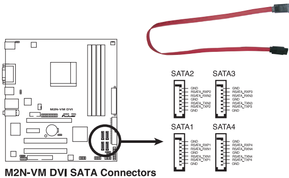
M2N-VM DVI SATA Connectors
