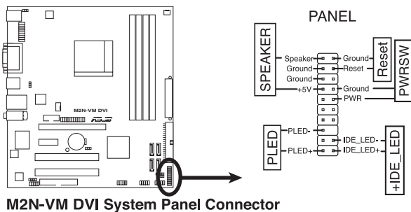
M2N-VM DVI System Panel Connector
