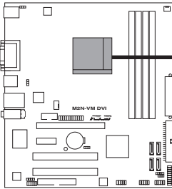
M2N-VM DVI CPU Socket AM2
