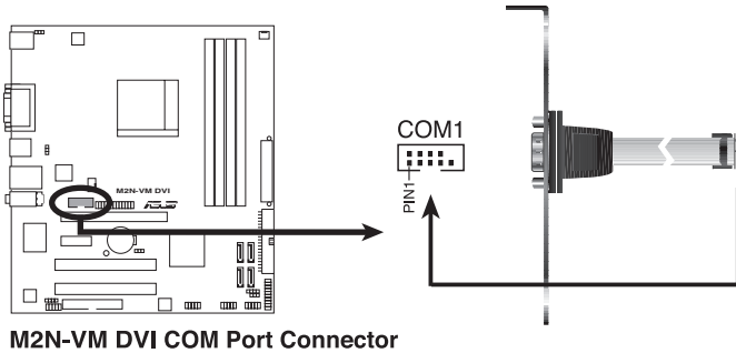
M2N-VM DVI COM Port Connector
