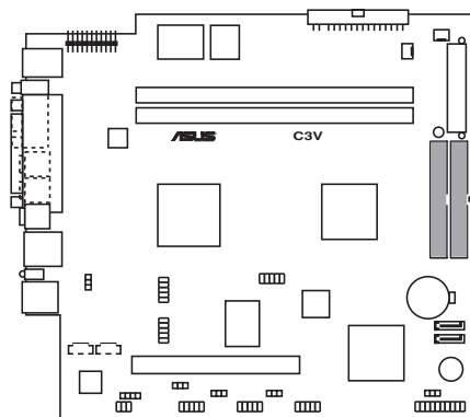
C3V IDE connectors
