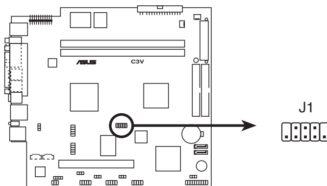
C3V TV-out/S-Video out connector
