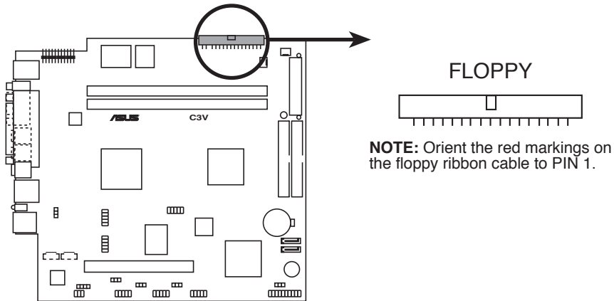
C3V Floppy disk drive connector
