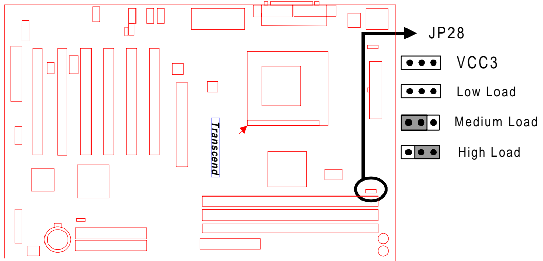
VCC3 Adjust
