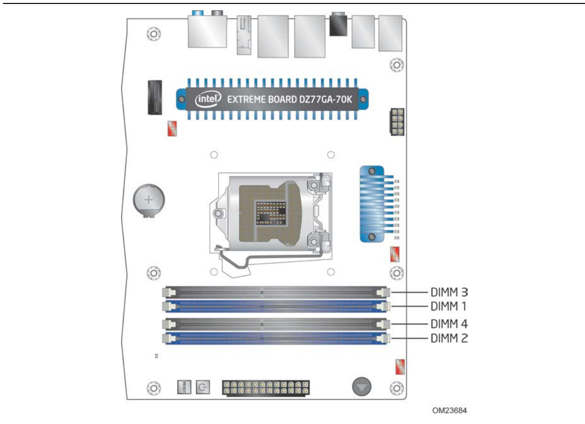
Figure 3. DIMM Configuration
