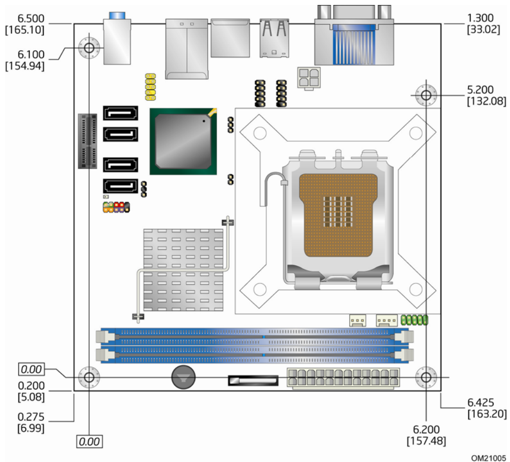
Figure 14. Board Dimensions
