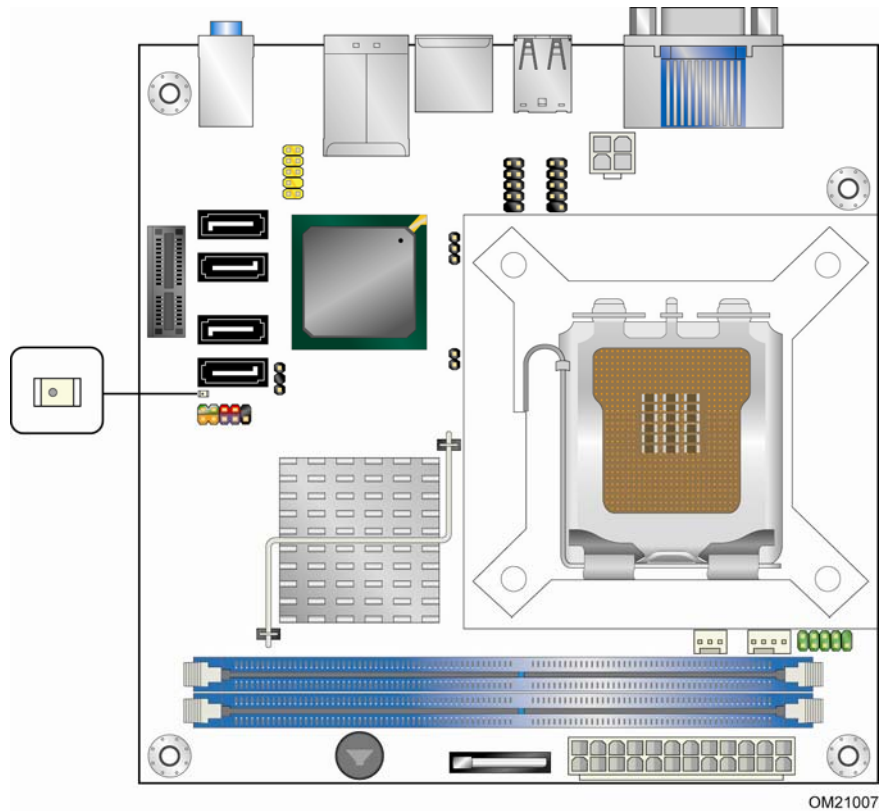
Figure 7. Location of the Standby Power Indicator LED
