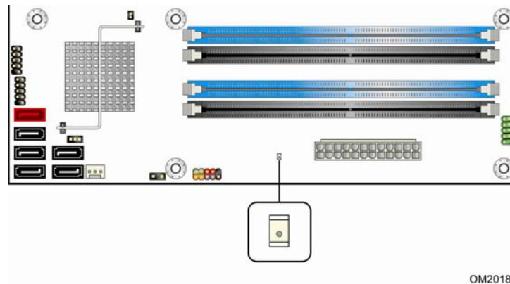
Figure 8. Location of the Standby Power Indicator LED
