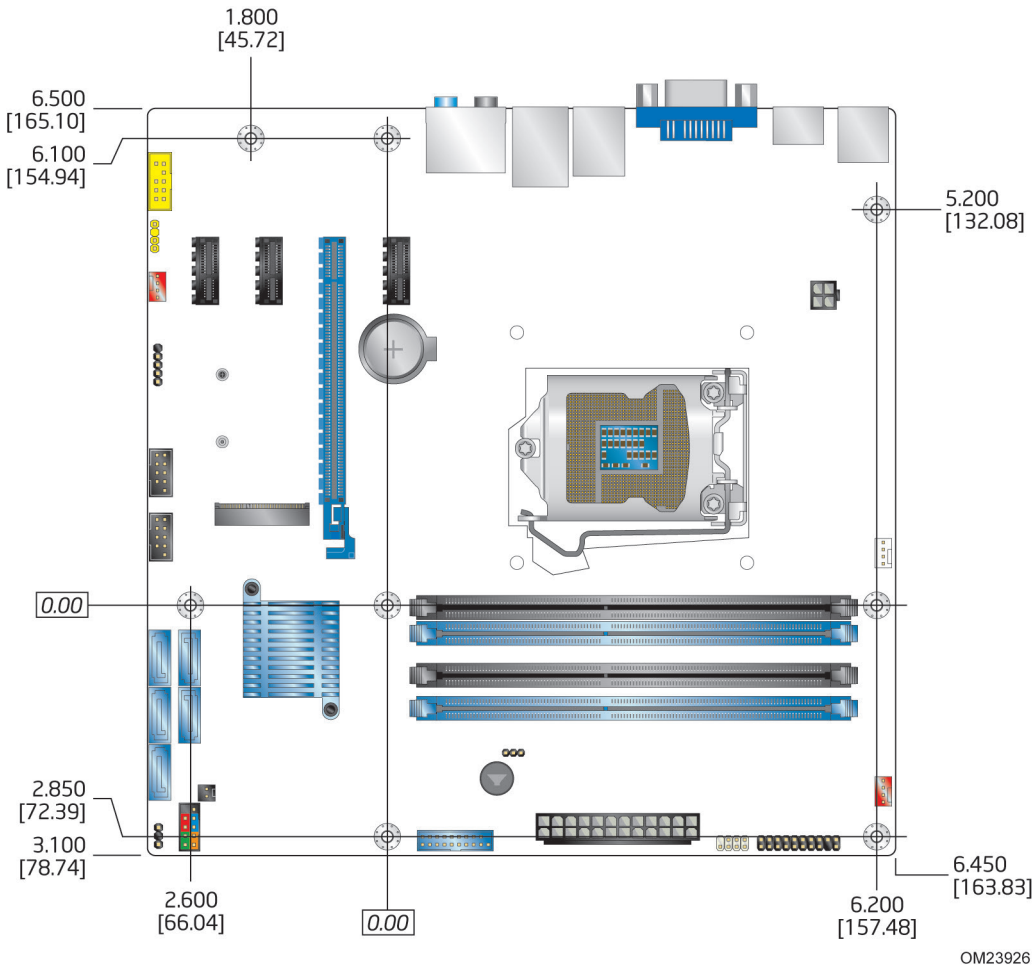
Figure 15. Board Dimensions
