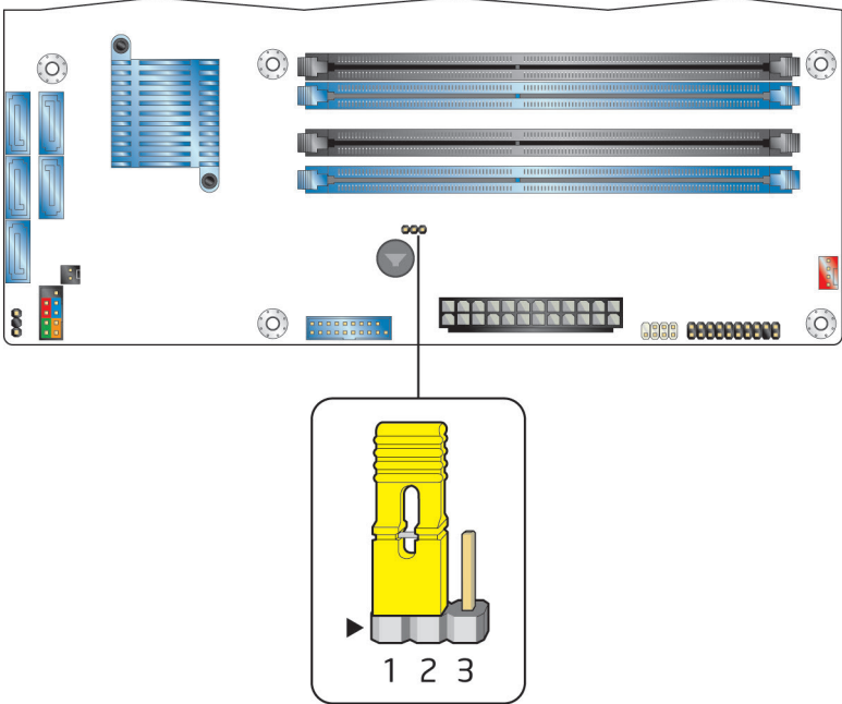
Figure 14. Location of the Jumper
