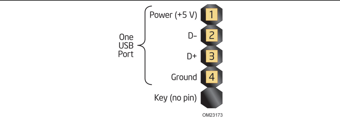
Figure 12. Connection Diagram for the Front Panel USB 2.0 Single-Port Header
