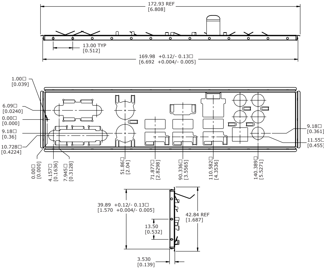
Figure 22. I/O Shield Dimensions for Boards with PS/2 Connectors
