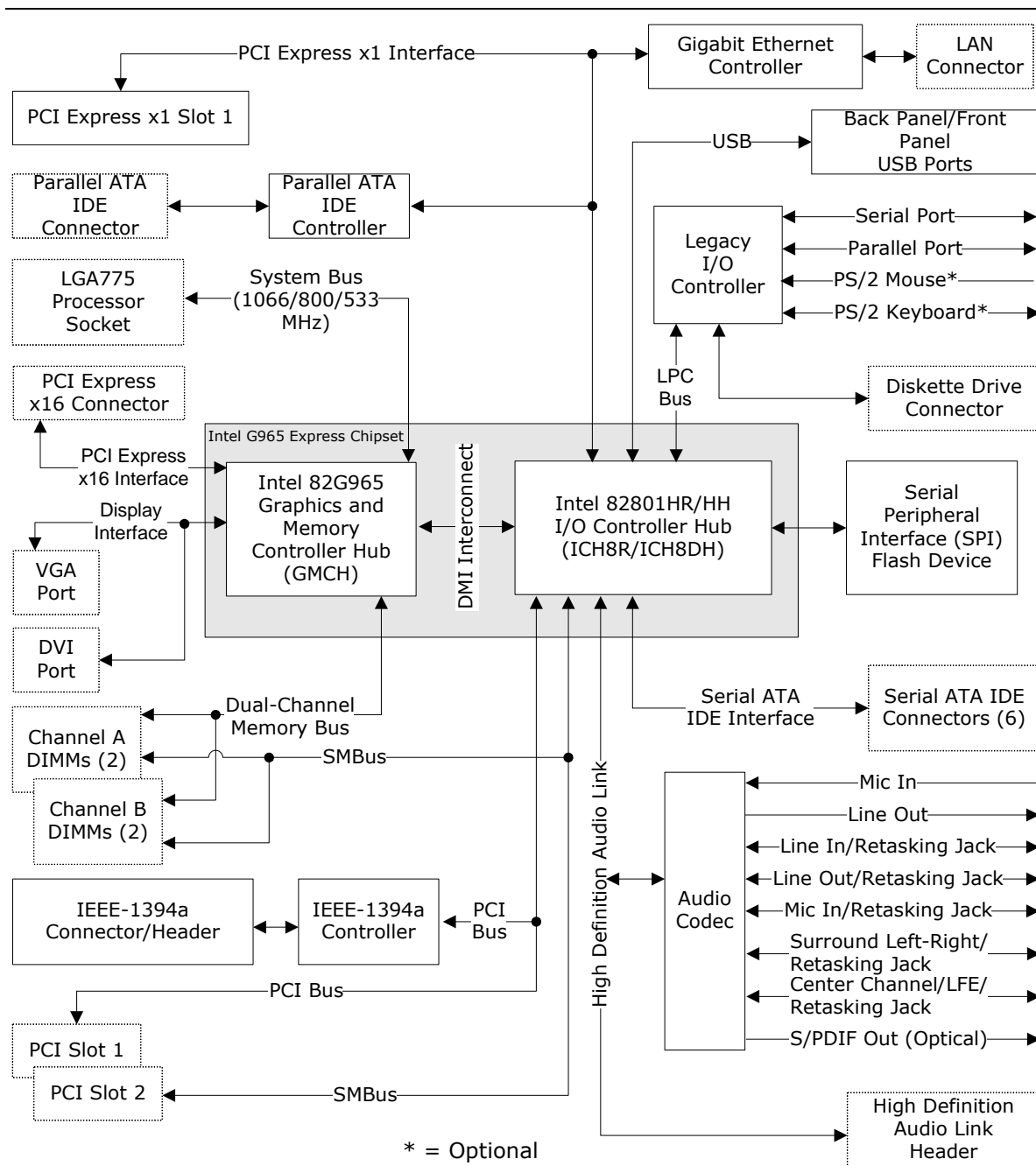
Figure 2. Block Diagram
