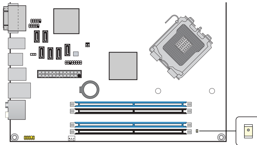
Figure 13. Location of the Standby Power Indicator LED
