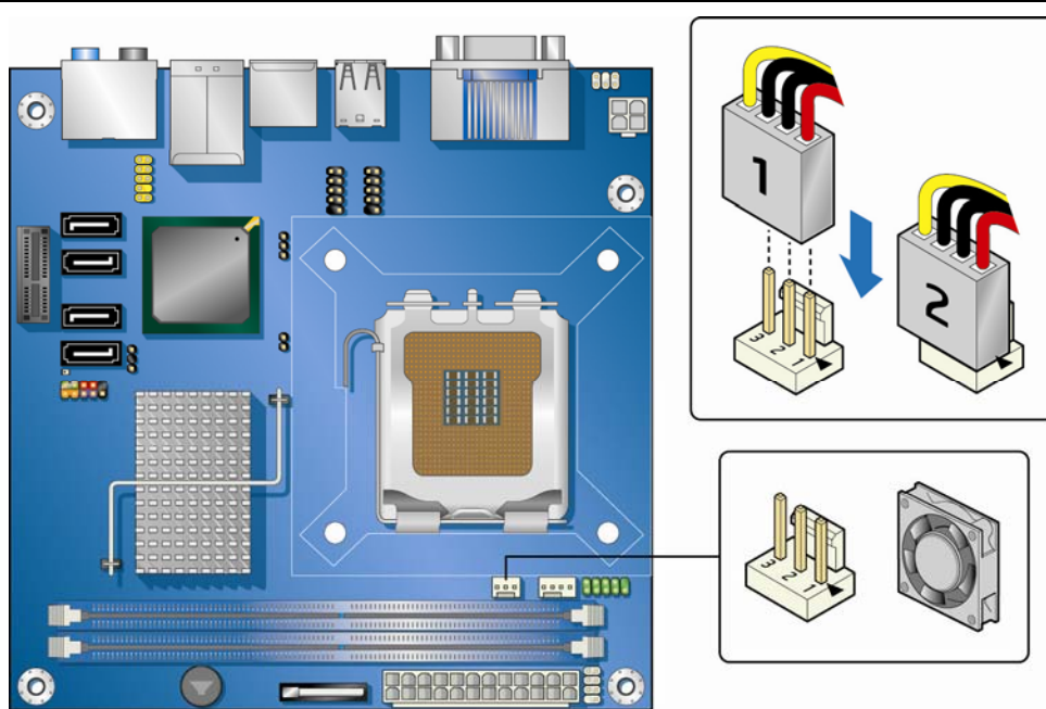
Figure 19. Location of the Chassis Fan Headers
