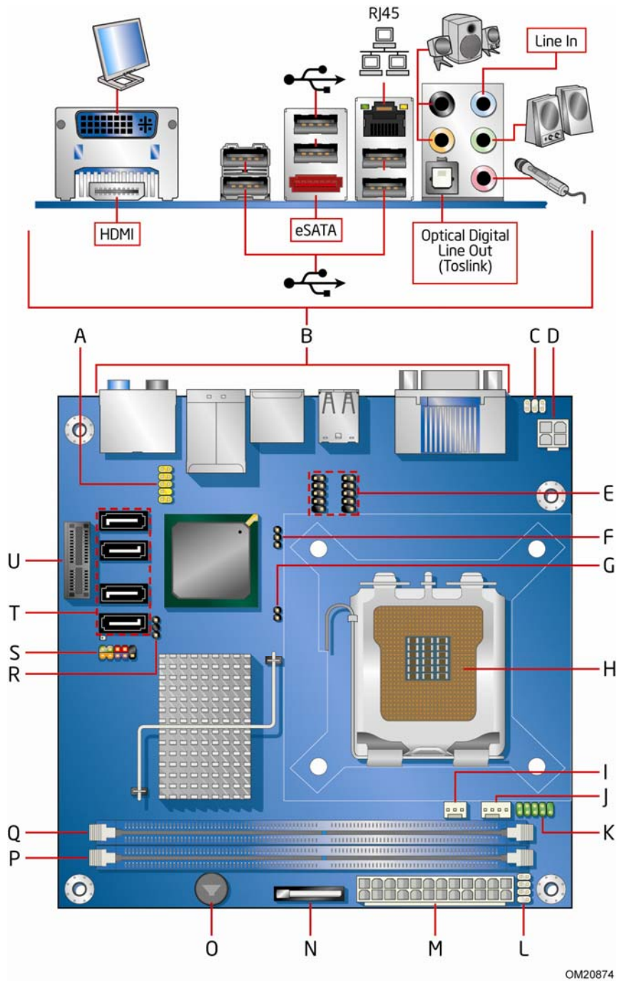
Figure 1. Desktop Board DG45FC Components
