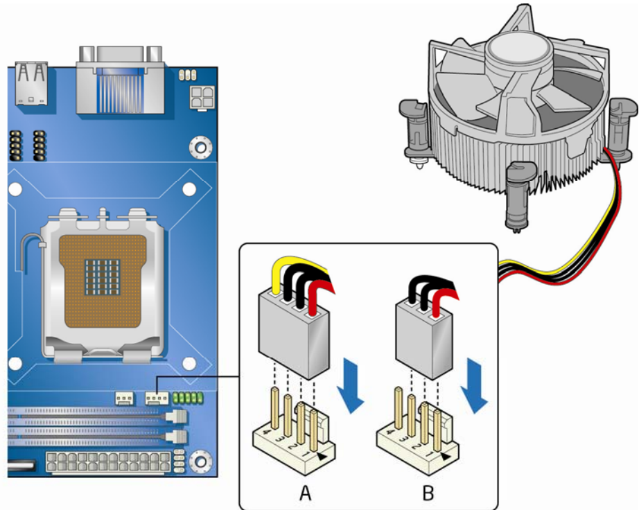
Figure 12. Connecting the Processor Fan Heat Sink Cable
