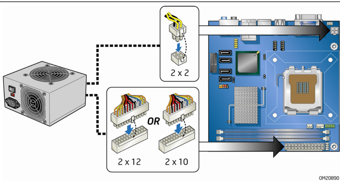
Figure 20. Connecting Power Supply Cables
