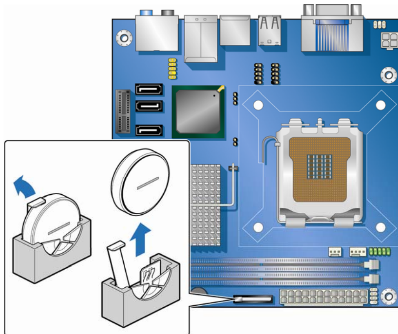
Figure 22. Removing the Battery
