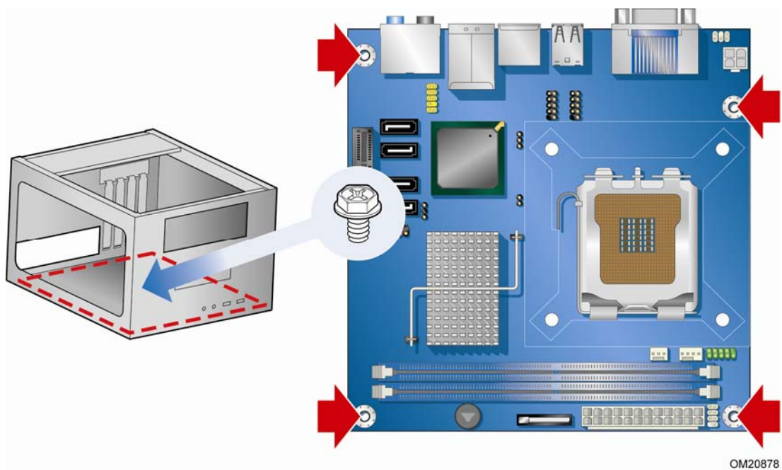
Figure 5. Desktop Board DG45FC Mounting Screw Hole Locations
