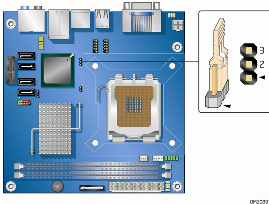
Figure 21. Location of the BIOS Configuration Jumper Block
