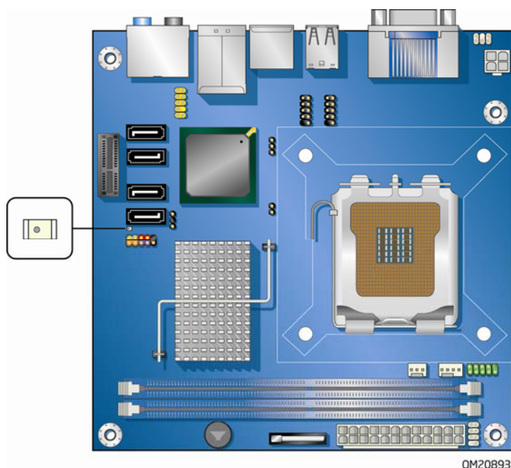
Figure 3. Location of the +5 V Standby Power Indicator
