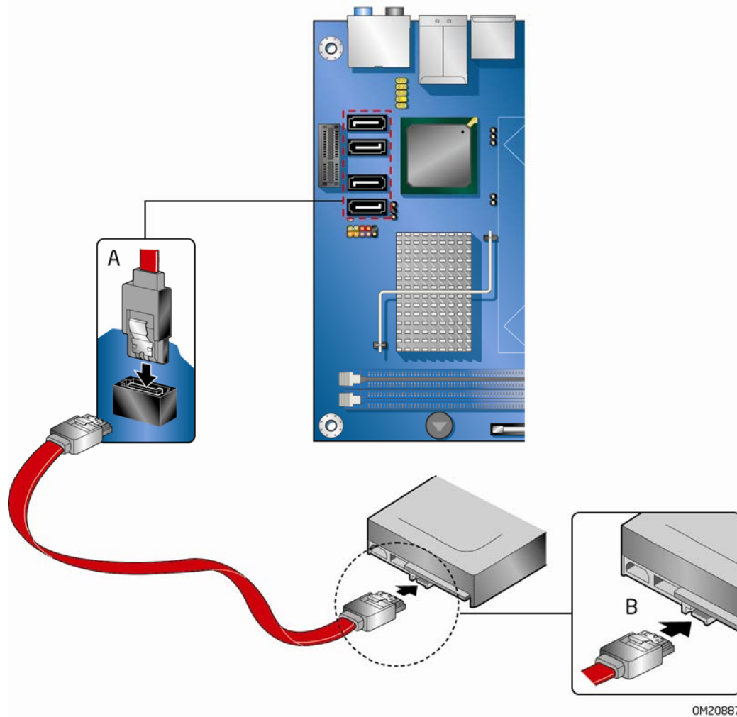
Figure 16. Connecting a Serial ATA Cable
