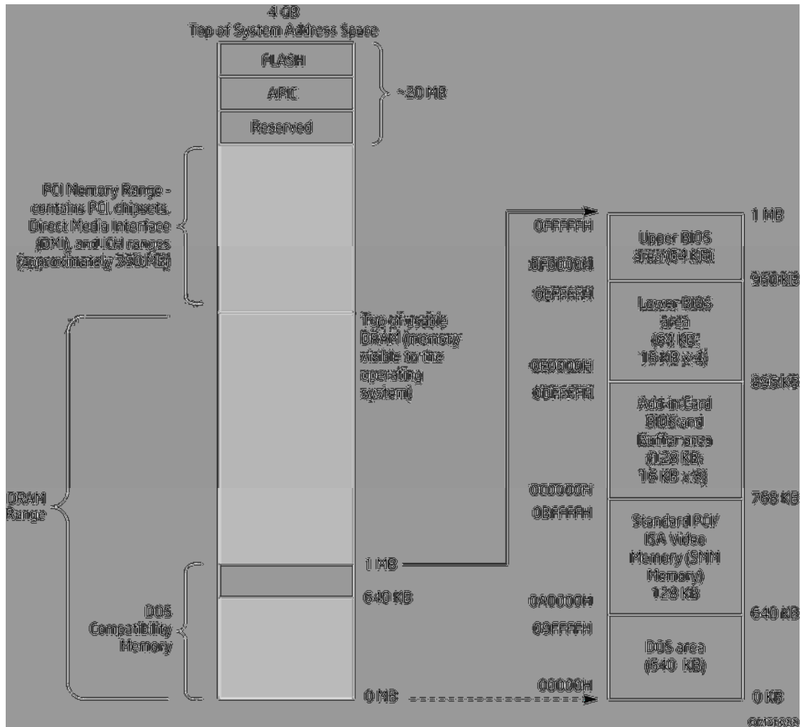
Figure 8. Detailed System Memory Address Map
