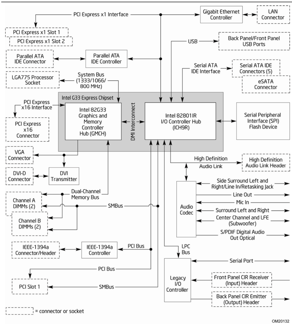
Figure 2. Block Diagram
