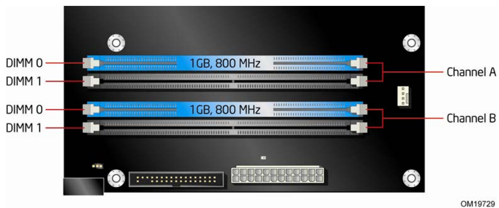
Figure 14. Dual Channel Memory Configuration Example 1
