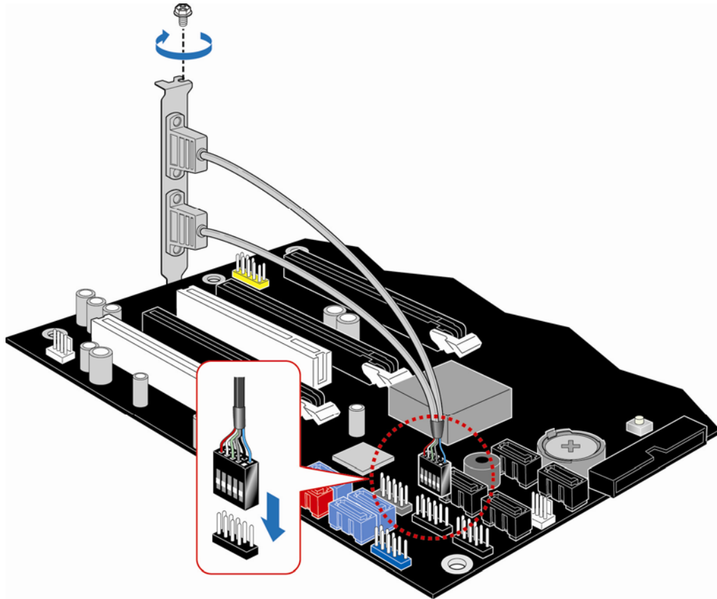
Figure 25. Connecting the Rear Panel USB 2.0 Adapter
