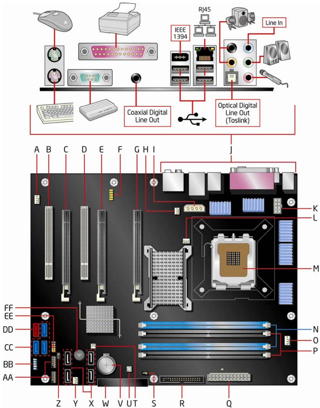
Figure 1. Desktop Board D975XB2 Components
