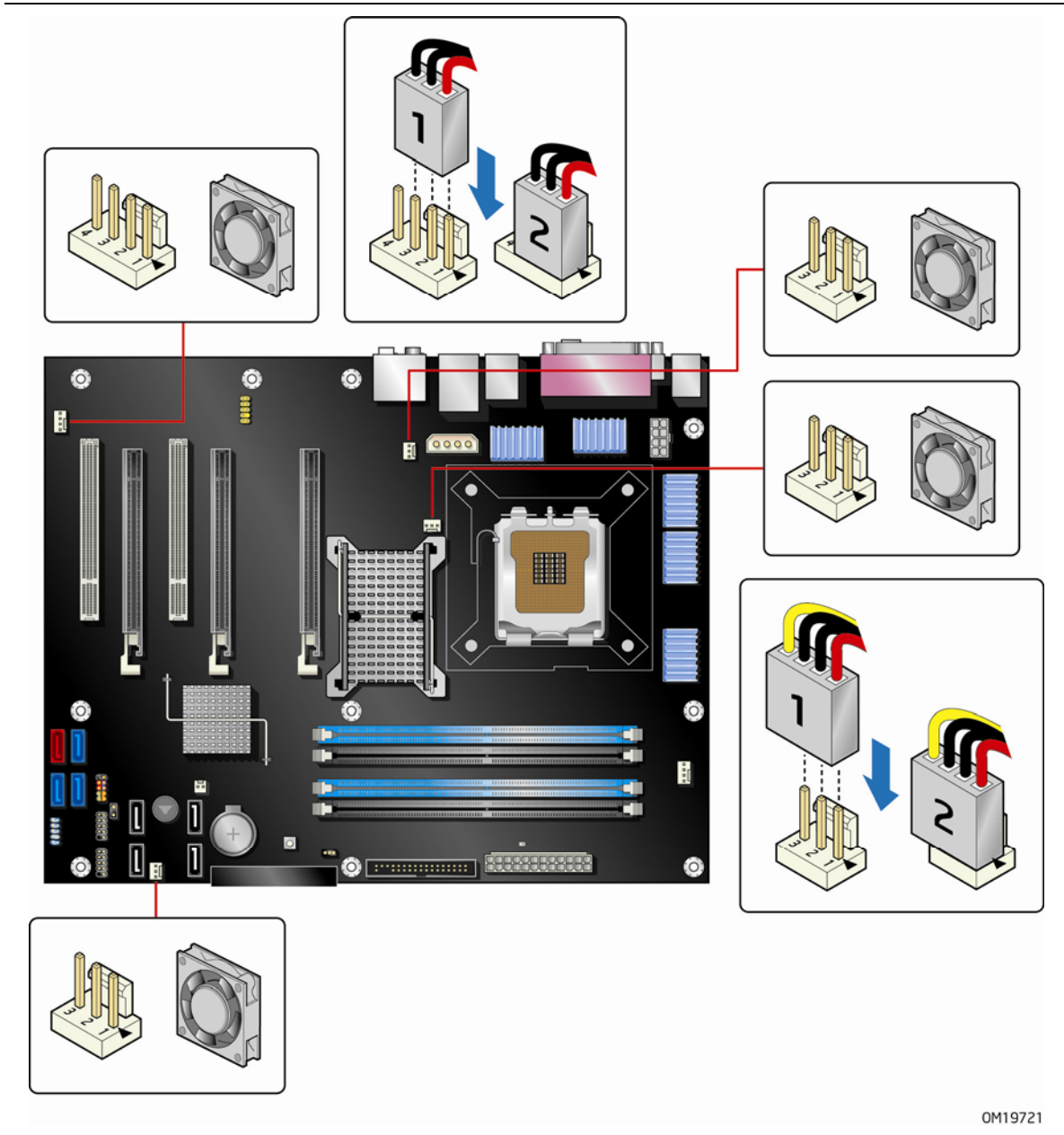
Figure 27. Location of Fan Headers
