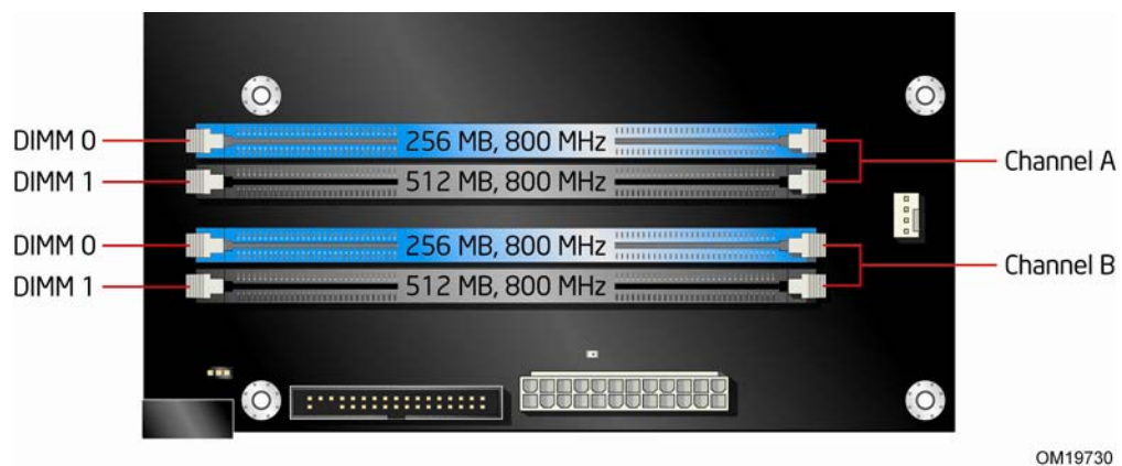
Figure 15. Dual Channel Memory Configuration Example 2
