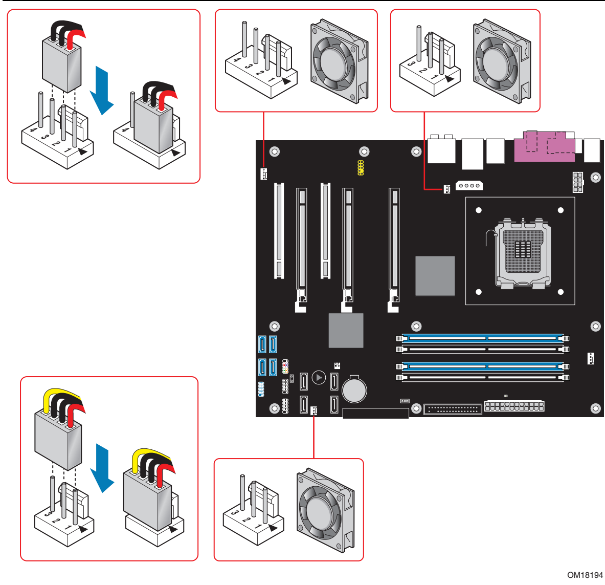
Figure 25. Location of Fan Headers
