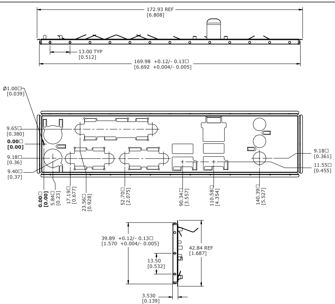
Figure 19. I/O Shield Dimensions
