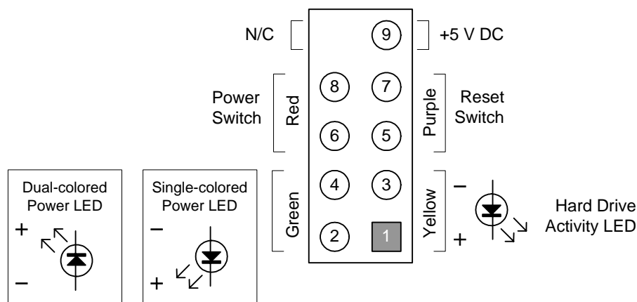
Figure 13. Connection Diagram for Front Panel Connector
