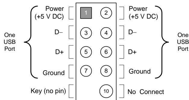
Figure 14. Connection Diagram for Front Panel USB Connectors
