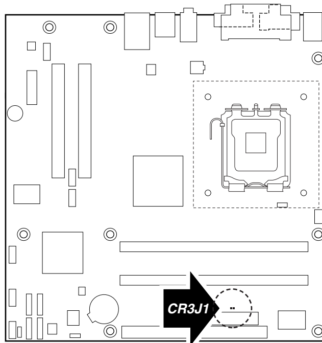
Figure 10. Location of the Standby Power Indicator LED
