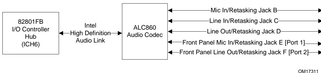
Figure 7. High Definition Audio Subsystem Block Diagram
