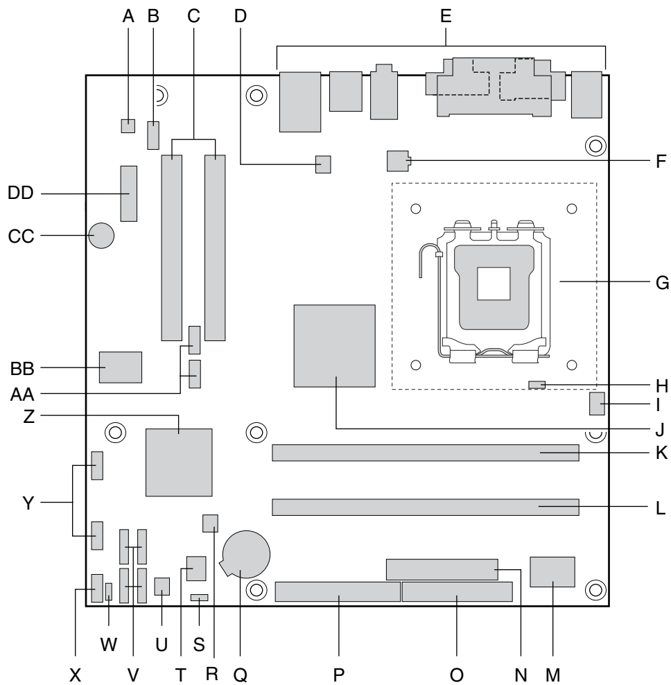
Figure 1. Board Components
