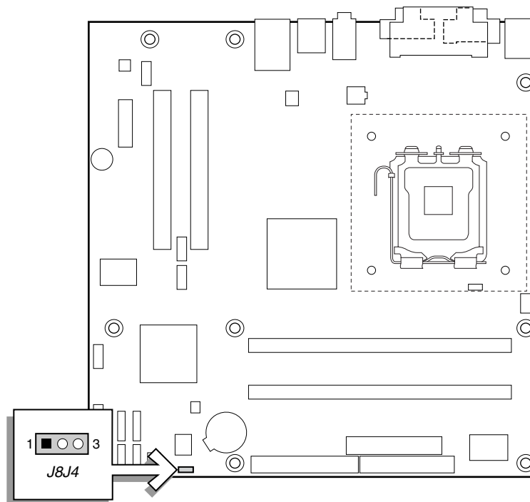
Figure 16. Location of the Jumper Block
