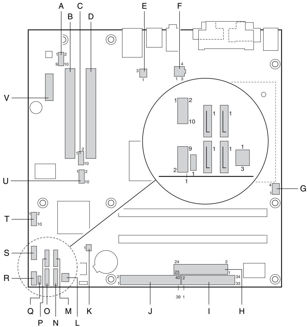
Figure 12. Component-side Connectors
