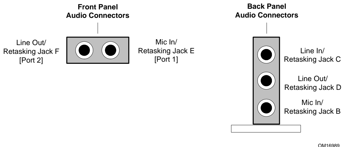
Figure 6. Front/Back Panel Audio Connector Options for High Definition Audio Subsystem
