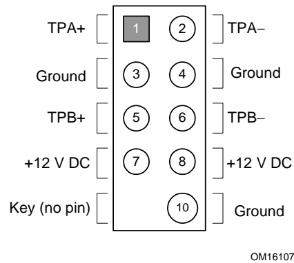
Figure 15. Connection Diagram for IEEE 1394a Connector
