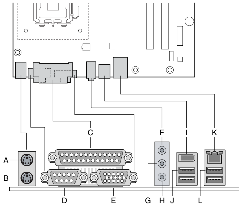
Figure 11. Back Panel Connectors
