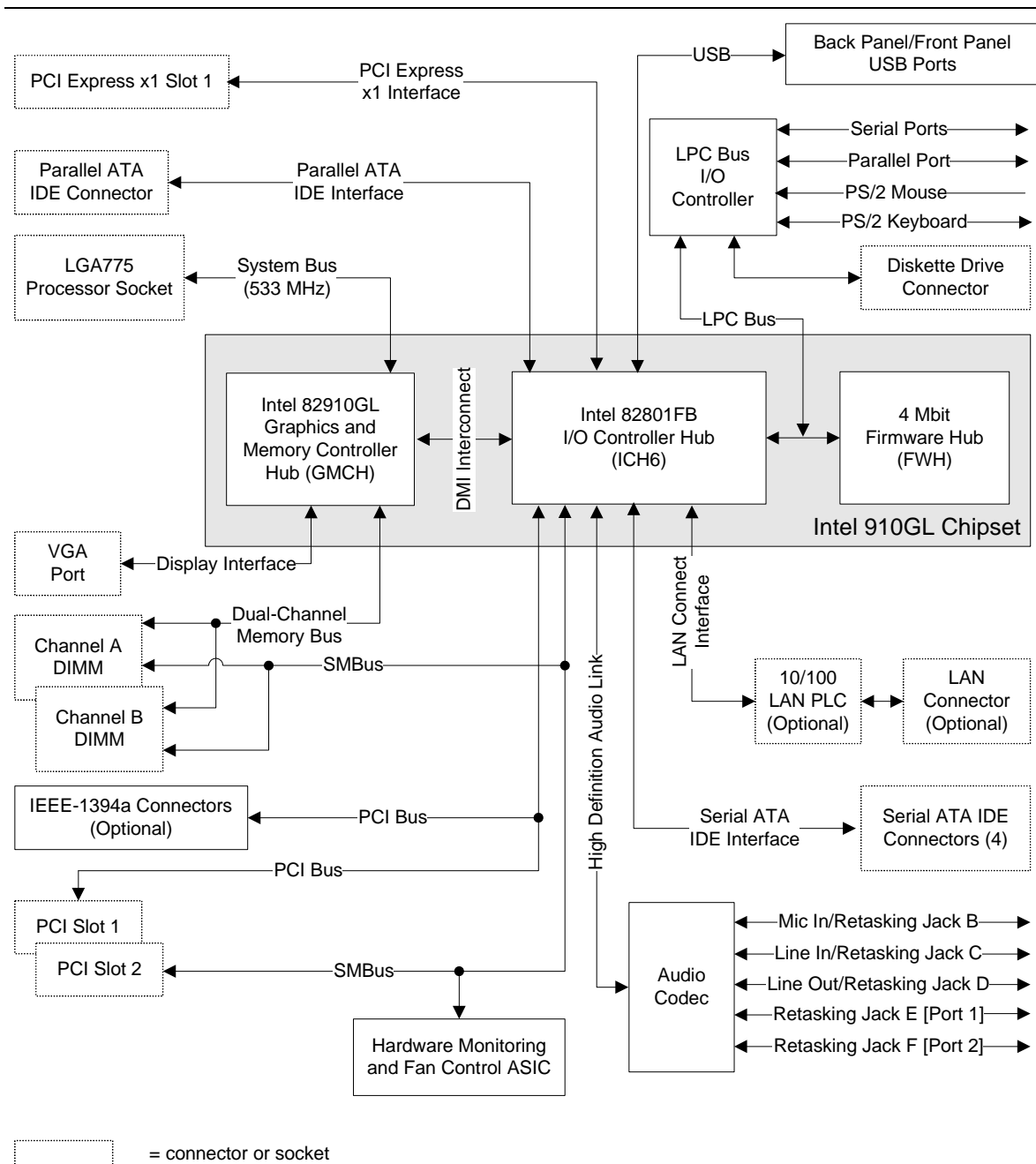
Figure 2. Block Diagram
