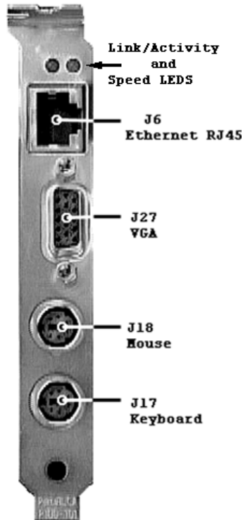
Figure 1-3 Captor 370 Bracket
