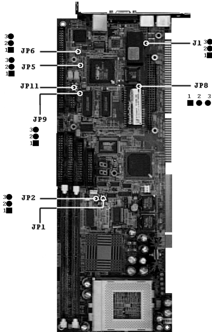
Figure 1-2 Jumper Locations - Front
