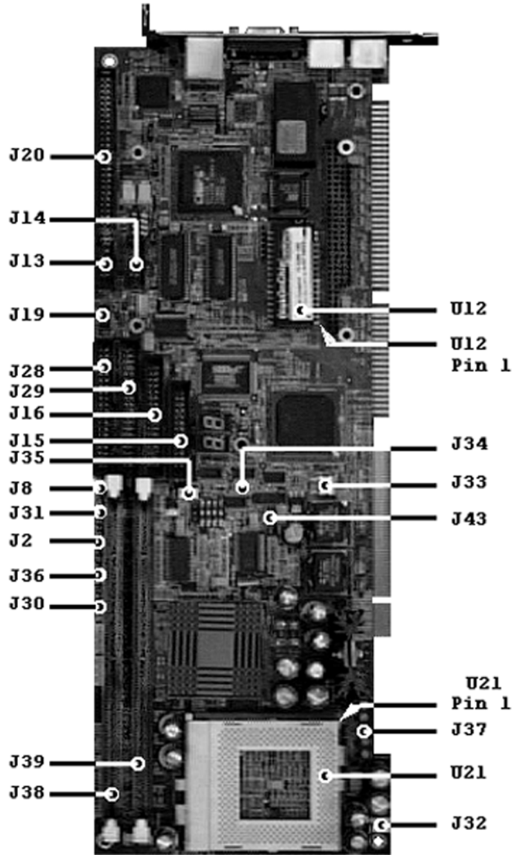
Figure 1-4 Location of Components and Header Connectors
