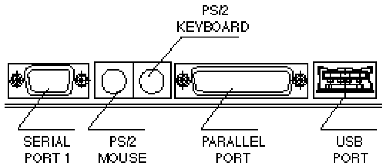
Figure 2-2 External connectors
