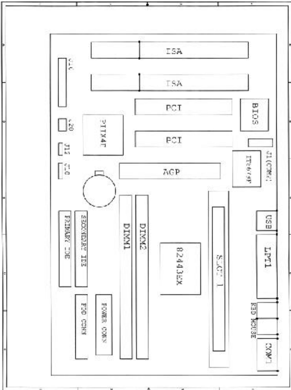
Figure 1-1. CB644M-EX Motherboard Layout
