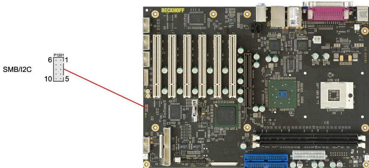
Pinout SMBus/I2C connector:
