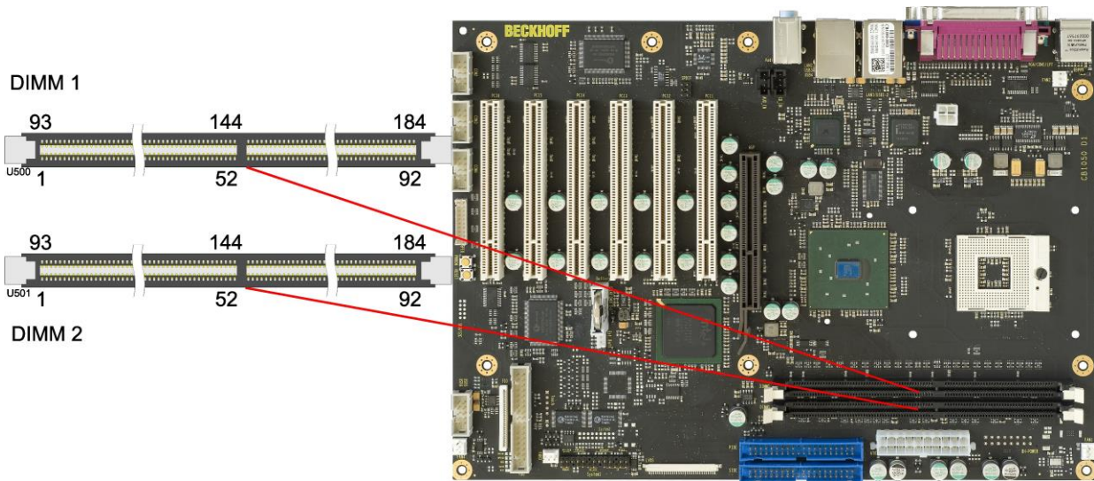
Pinout DIMM184-DDR:
