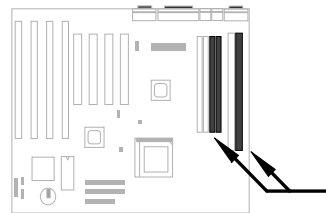
Double side module at either Bank1 or DIMM2, the other must be empty.
